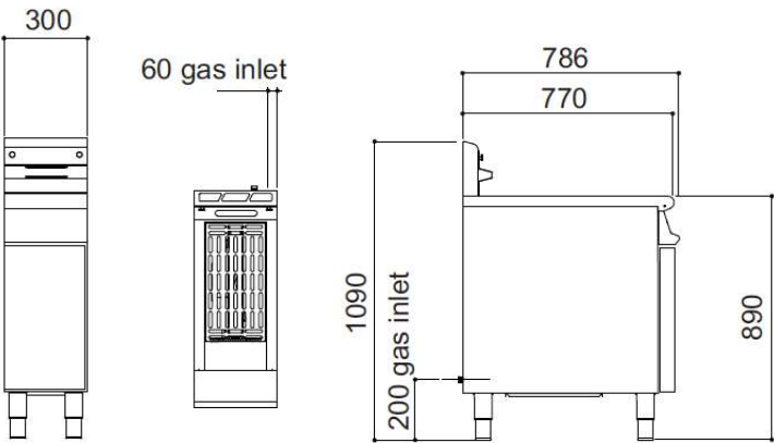
Measurements in mm Unit on castors is the same hob height
